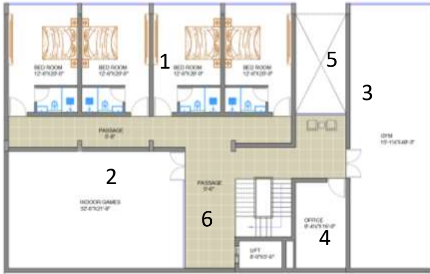
FIRST FLOORPLAN
